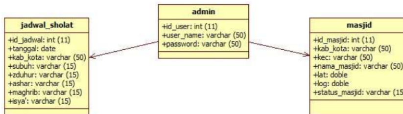
Gambar 6 Class Diagram
