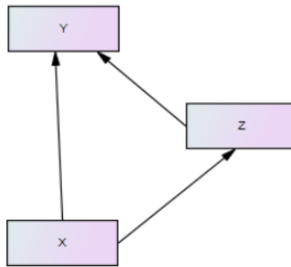
Gambar 1. Path Analysis
