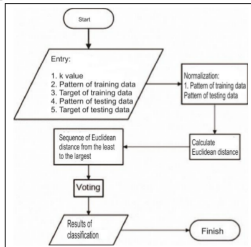
Fig. 3. kNN algorithm flowchart
